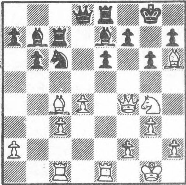
356 After 21...Rc7
